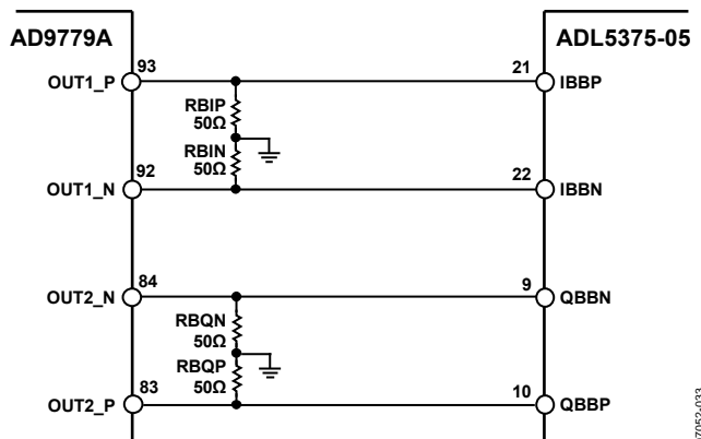
Figure 57. Interface Between the AD9779A and ADL5375-05 with 50 Ω Resistors to Ground to Establish the 500 mV DC Bias for the ADL5375-05 Baseband Inputs
